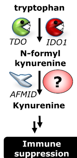
Fig. 1. Kynurenine pathway
