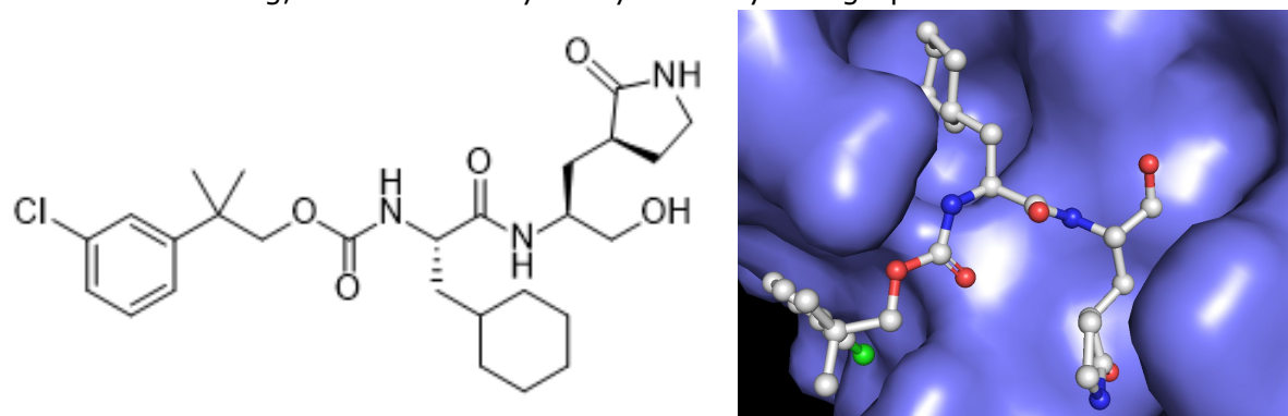
Figure 1. Example of peptidomimetic norovirus protease inhibitor [1] . Left: 2D chemical structure. Right: crystal structure of the inhibitor bound in the active site of norovirus NS6 pro (image generated on PyMol).
